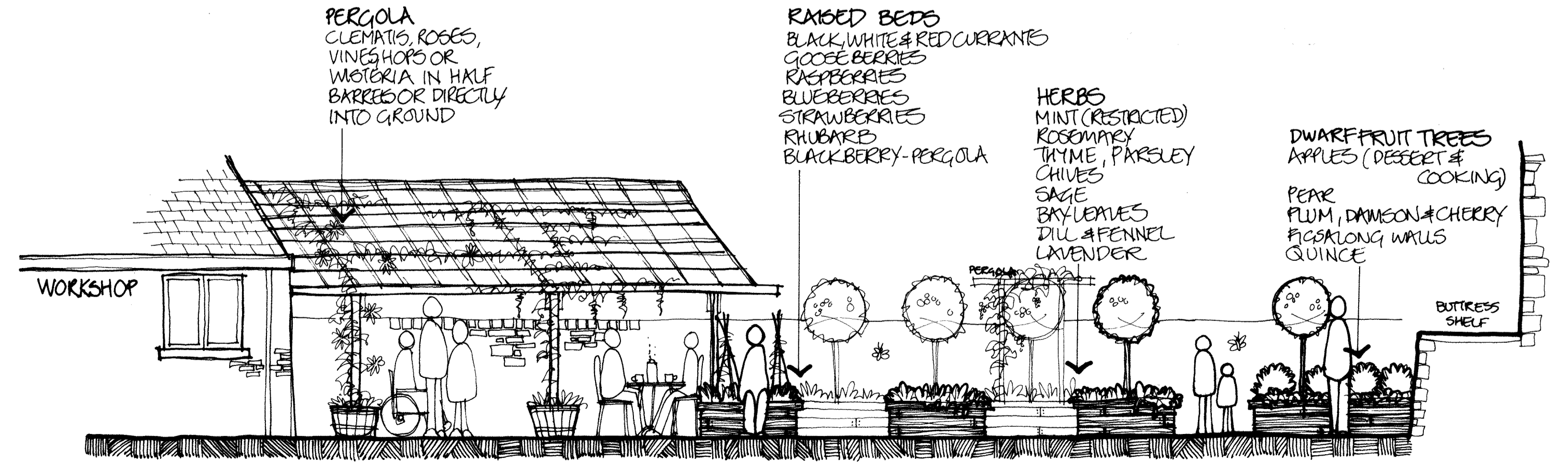
SECTION THROUGH RAISED BED AREA 1:50
